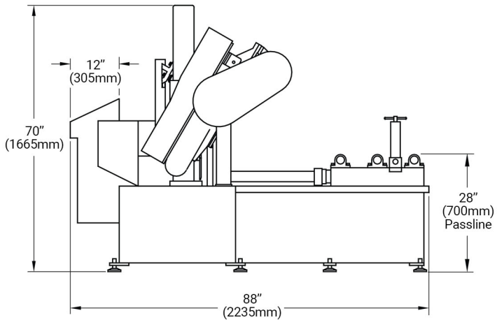
Dimensional Drawings of DC-420NC
