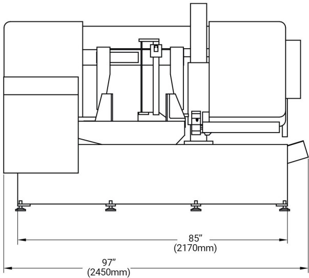
Dimensional Drawings of DC-420NC
