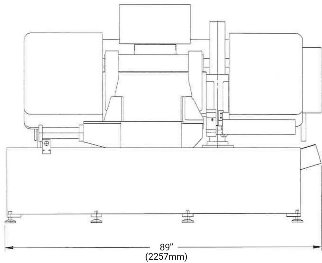
Dimensional Drawings of DC-330SA
