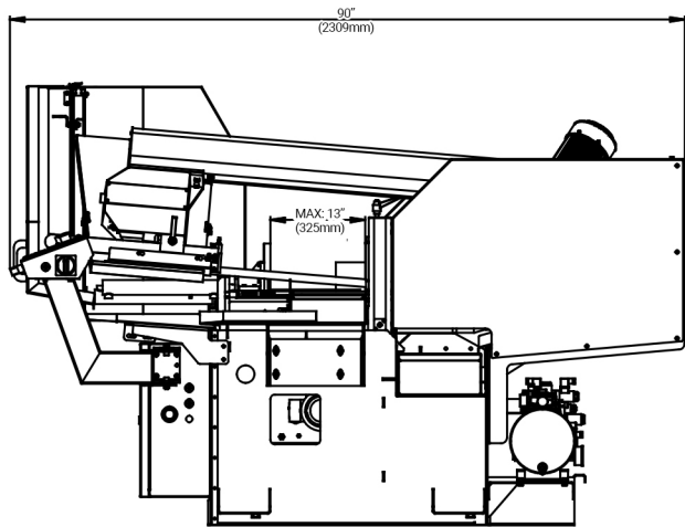
Dimensional Drawings of S-320CNC
