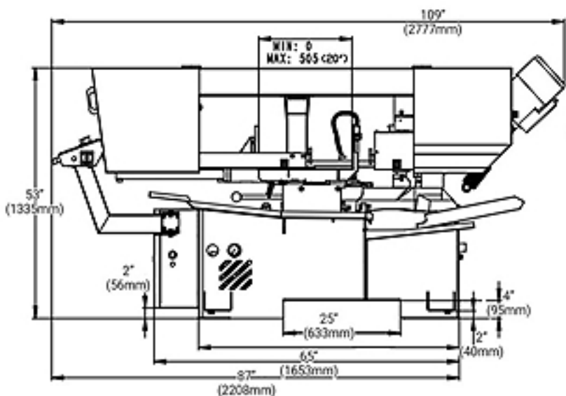
Dimensional Drawings of DS-500SA
