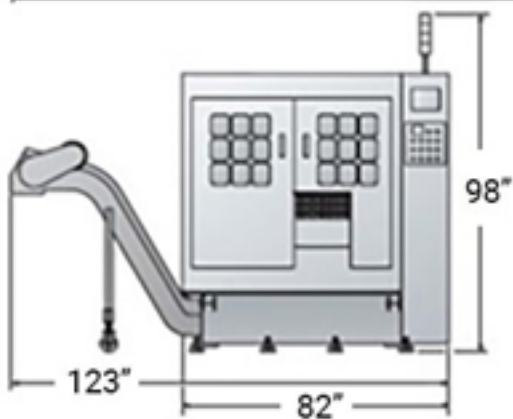
Dimensional Drawings of SC-150A
