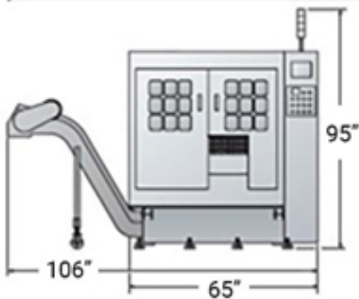
Dimensional Drawings of SC-75A
